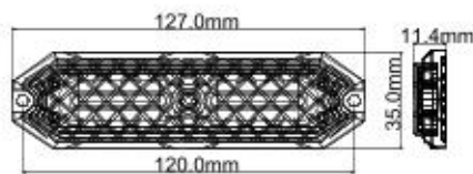
LED-20035-6
