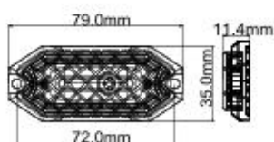
LED-20035-3
