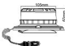
WL400PRO
