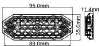
LED-20035-4
