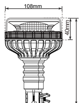
WL1233NB-SF Flexible base with screwing cap
