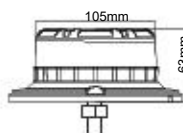
WL401PRO-BO
