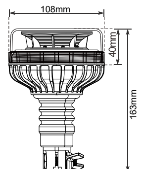
WL834NB-SMC-SF Flexible base with screwing cap
